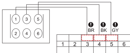
Terminal block 3 (Indoor Unit)
